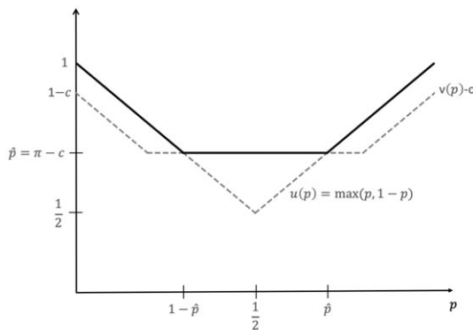
FIGURE 2.—Binary signals with precision \pi .
