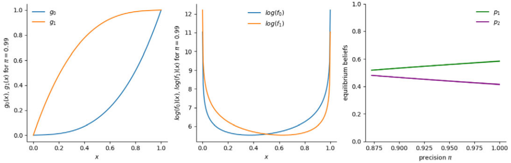
FIGURE 4.—Transition functions, densities, and beliefs for n = 3 .
