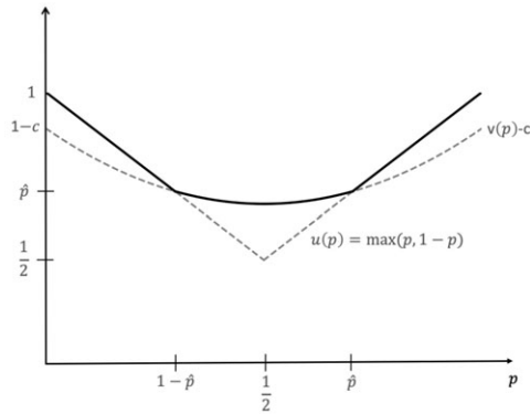
FIGURE 1.—Signals with unbounded strength.
